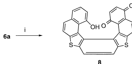
Scheme 2. Reagent and conditions: i, ( n -Bu) 4 NF, THF.
